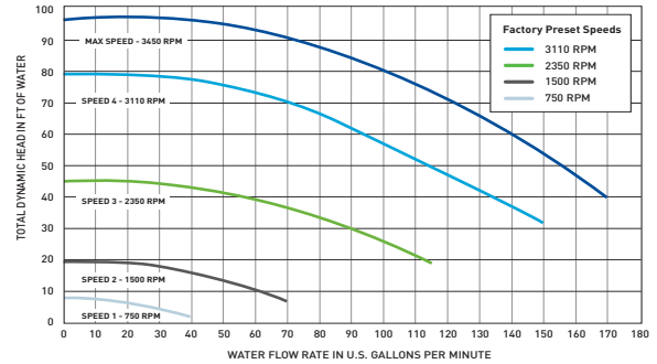
NOTE: The chart above demonstrates performance rates at factory preset speeds of 750 RPM, 1500 RPM, 2350 RPM and 3110 RPM.
