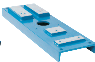
FABRICATED STEEL Economical baseplate that meets ANSI/ASME B73.1 M current edition dimensional requirements.
