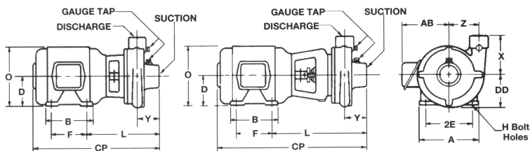
STANDARD MECH. SEAL
